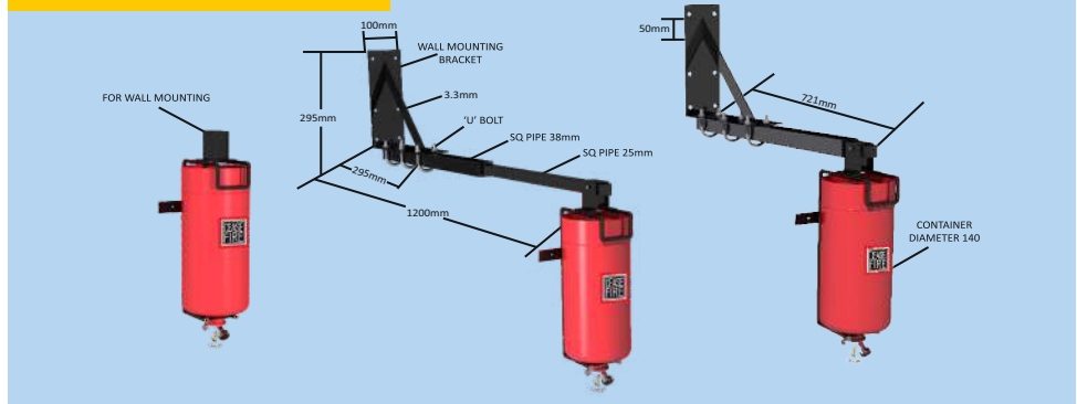
Fluoroketone Extinguishers [FK-5-1-12]
